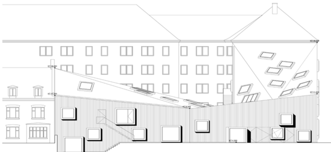
Principudformning for facade mod nord
