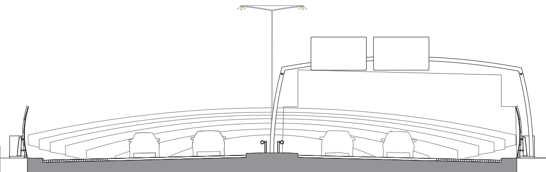
snit C 1:200
