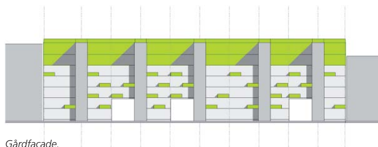
Gårdfacade.
